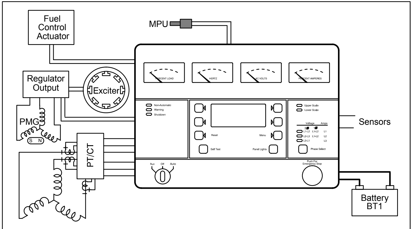
FIGURE 1-1. GENERATOR SET CONTROL FUNCTIONS
