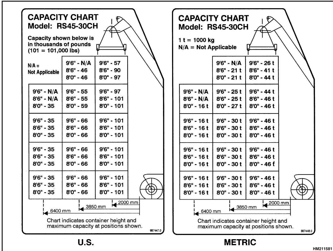
Figure 2. Lifting Capacities, Container Spreader
