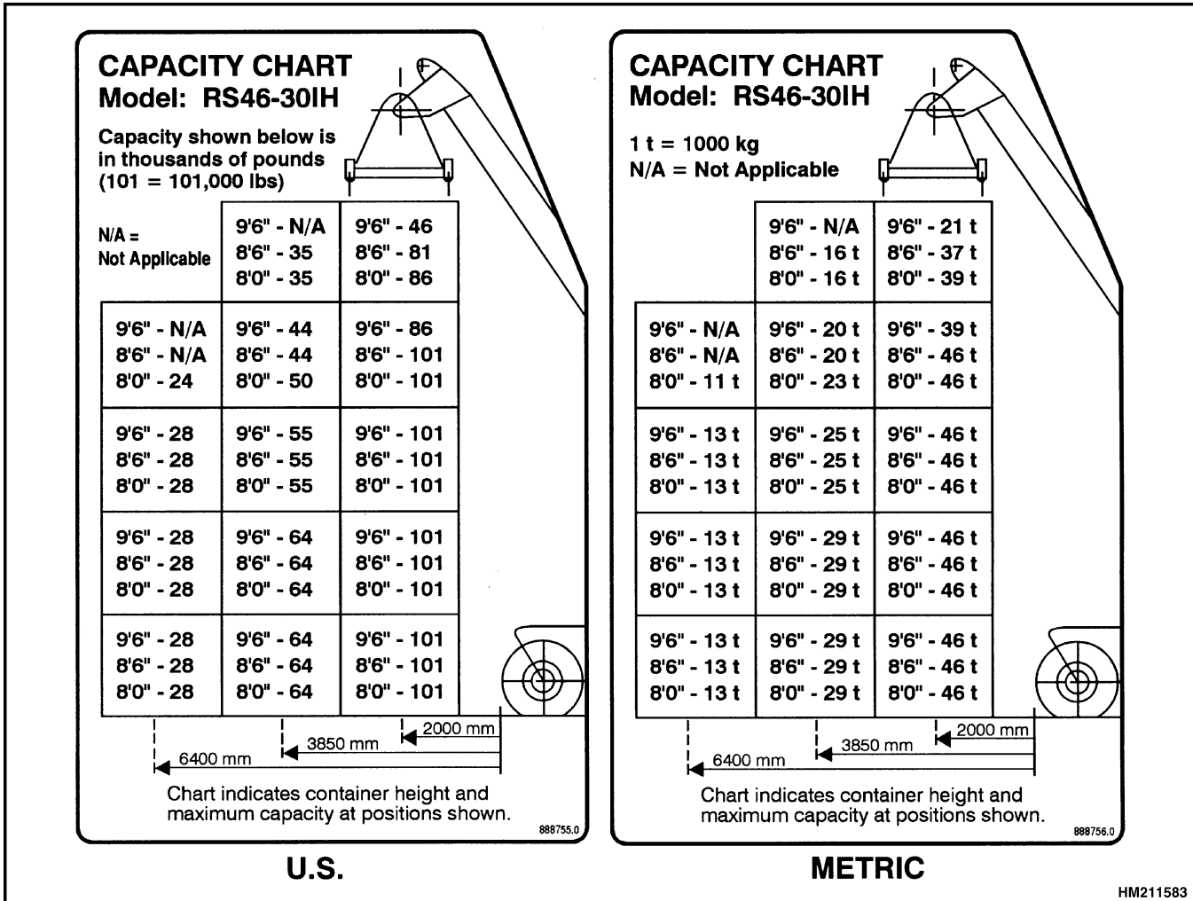
Figure 4. Lifting Capacities, Intermodal Spreader
