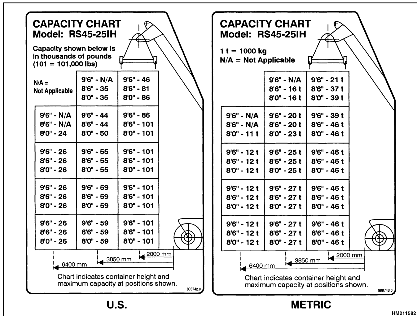
Figure 3. Lifting Capacities, Intermodal Spreader
