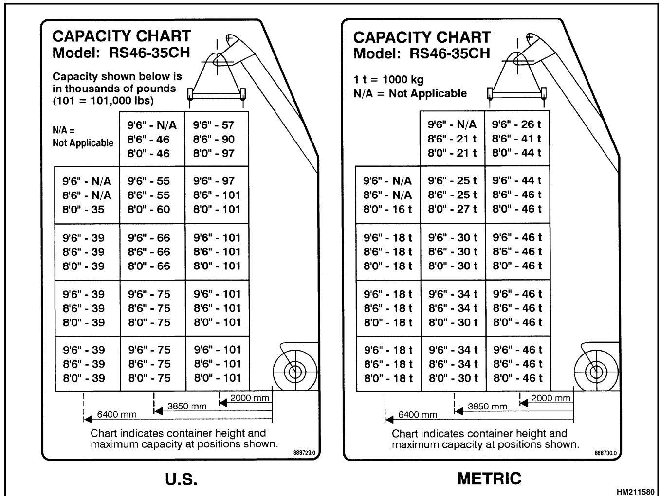
Figure 1. Lifting Capacities, Container Spreader
